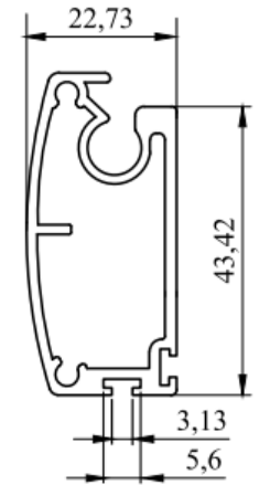
Bottom rail
